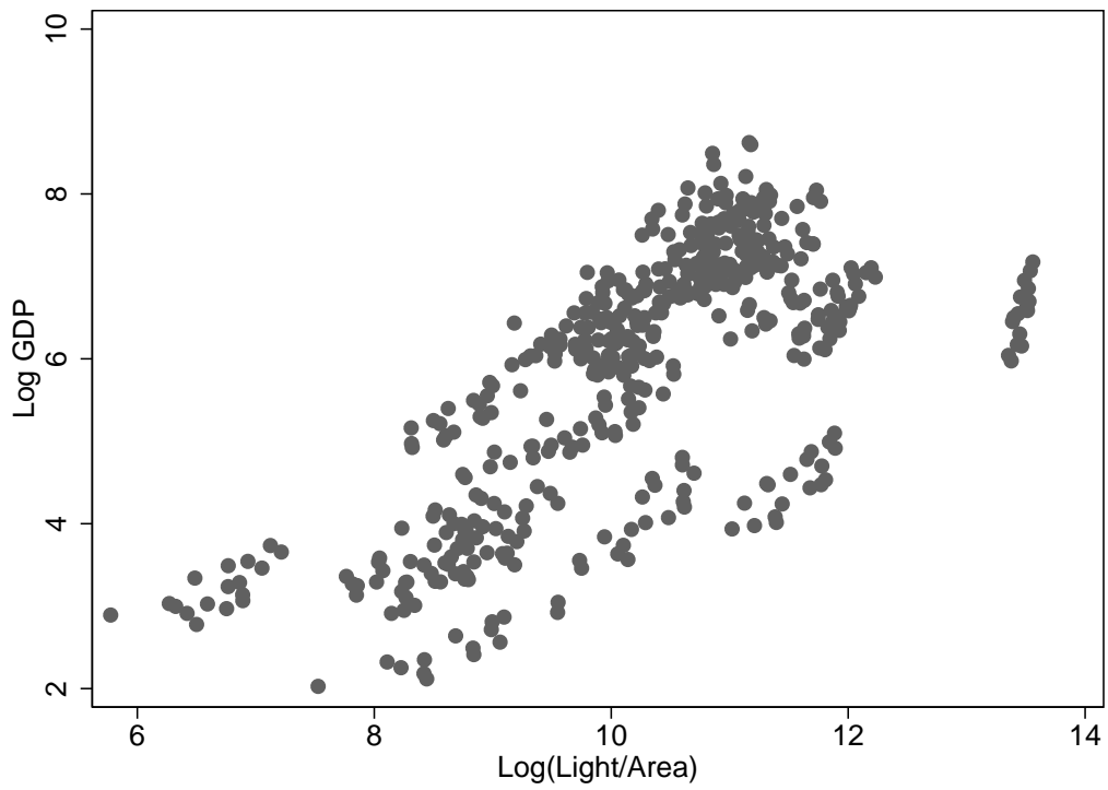
Figure A.1: Scatter of GDP against Night Light Luminosity: State data Note: \text{Log}(\text{Light}/\text{Area}) is the natural log of total light output of a state in a given year divided by its geographical area. \text{Log}(\text{GDP}) is the natural log of real GDP for each state. The time period is 1992-2009.
