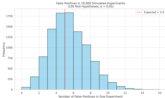
Figure 2. 100 hypotheses
